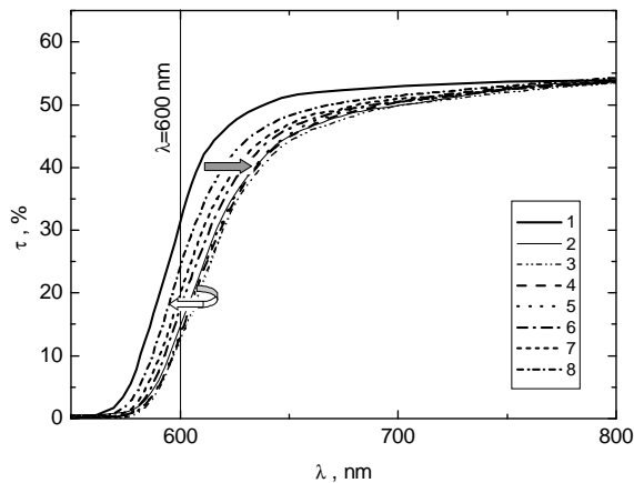
Fig. 2. Optical transmission spectra of the v\text{-As}_2\text{S}_3 ( d=1 mm) before (curve 1) and after (curve 2) \gamma -irradiation ( \Phi=10.0 MGy, P=25 Gy/s), as well as with further thermal annealing at 330 (curve 3), 370 (curve 4), 380 (curve 5), 395 (curve 6), 420 (curve 7) and 440 K (curve 8).
