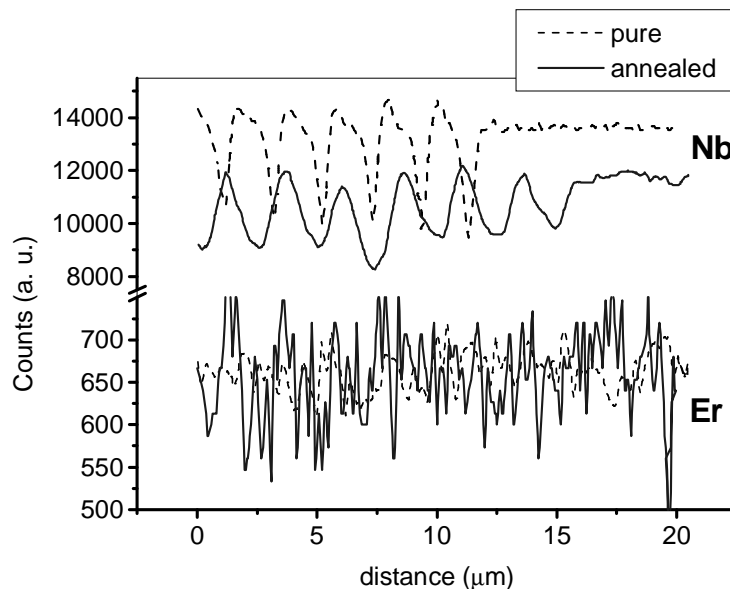
Fig. 3. WDX profiles measured along an Er:PPLN sample before (a) and after (b) an annealing process.
