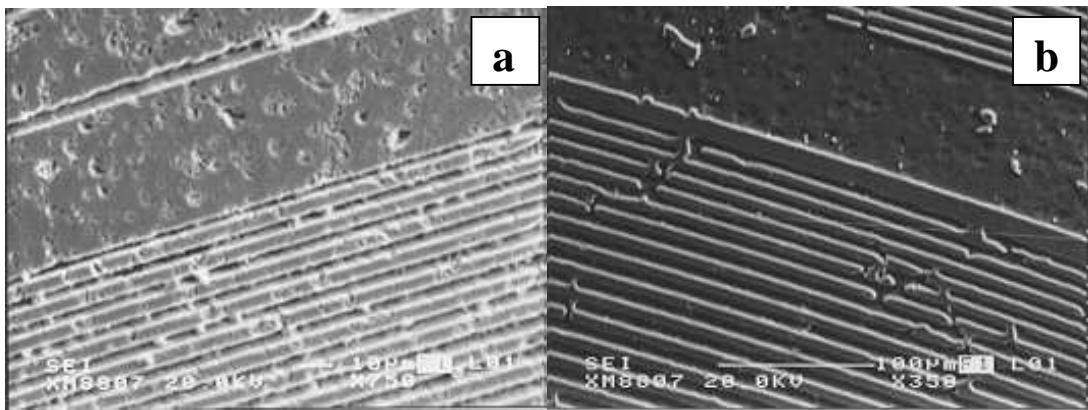
Fig. 1. Periodic structure of the tailored LN domain samples after removing about 1\mu\text{m} of the surface after an annealing process at T > T_c followed by a slow cooling rate (a) and a quenching process (b).
