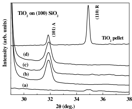
Fig. 5. XRD patterns of (a) an as-deposited TiO 2 thin film on SiO 2 and after successive annealing at (b) 600 °C, (c) 750 °C and (d) 1000 °C.
