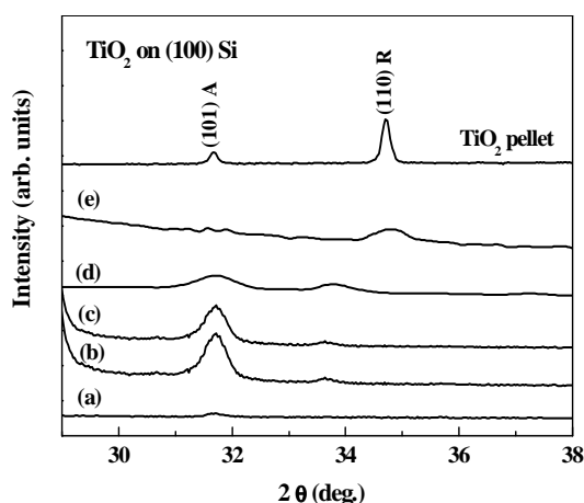
Fig. 4. XRD patterns of (a) an as-deposited TiO 2 thin film on Si and after successive annealing at (b) 600 °C, (c) 650 °C, (d) 750 °C, and (e) 1000 °C.
