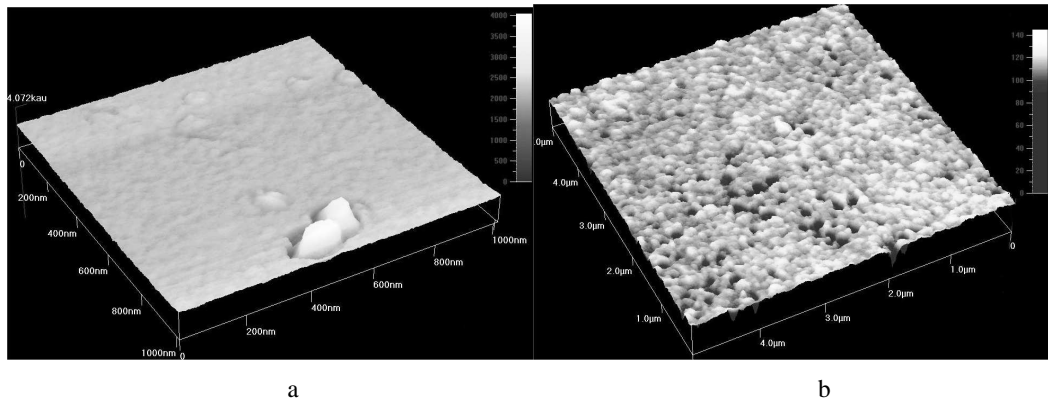
Fig. 1. Phase-mode AFM images of two TiO 2 thin films deposited on Si under (a) 1.6 mTorr and (b) 20 mTorr oxygen pressure.
