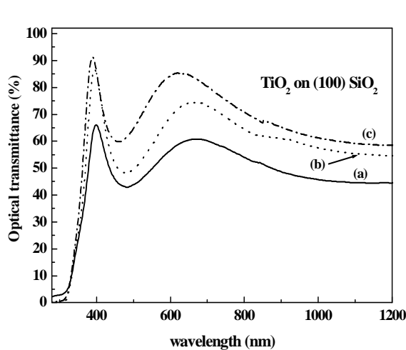
Fig. 7. Transmittance spectra of a TiO 2 thin film for (a) as-deposited, (b) annealed at 600 °C, and (c) annealed at 650 °C.
