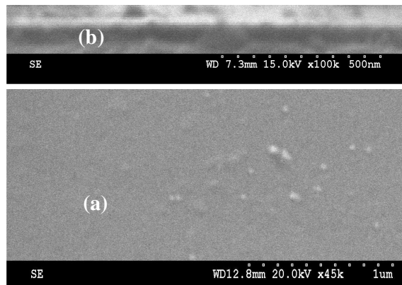
Fig. 2. (a) Cross-section and (b) surface SEM images of a TiO 2 thin film grown on Si.
