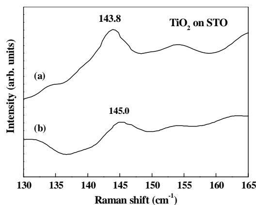
Fig. 6. Raman spectra of a TiO 2 thin film grown on STO for (a) as-deposited film and (b) annealed at 600 °C for 1h.
