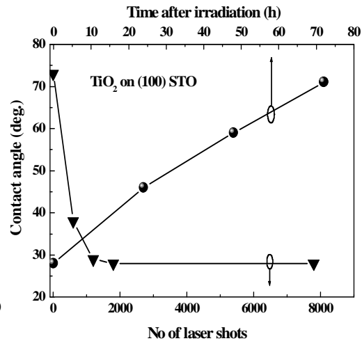
Fig. 8. Contact angle of a TiO 2 thin film as a function of number of laser shots during irradiation and as a function of time after post-irradiation.
