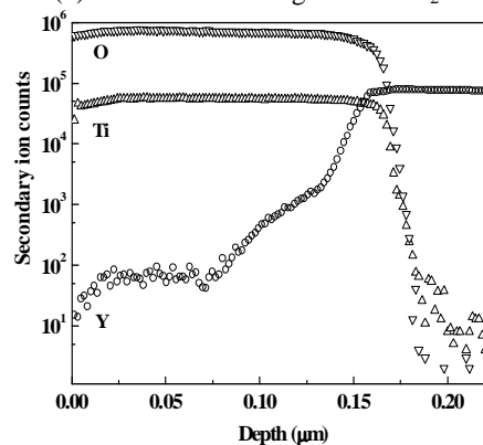
Fig. 3. A SIMS depth profile of a TiO 2 film grown on YSZ.
