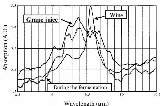
Fig. 10. Monitoring of the alcoholic fermentation process by using remote spectroscopy using a infrared fibre.
