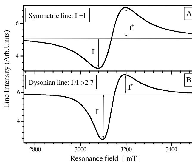
Fig. 2. The Electron Spin Resonance spectra of EBPANI at room temperature. a) The resonance spectra of symmetric pristine EBPANI; b) The Dysonian shape of the resonance line of EBPANI doped by 3% Cl/N.
