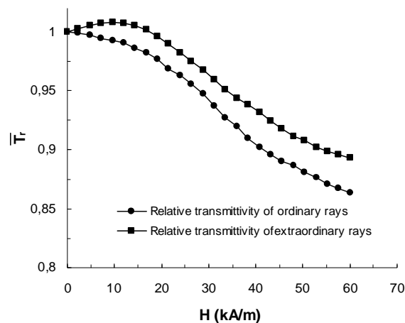
Fig. 3. The dependence of transmittivities of applied magnetic field strength.
