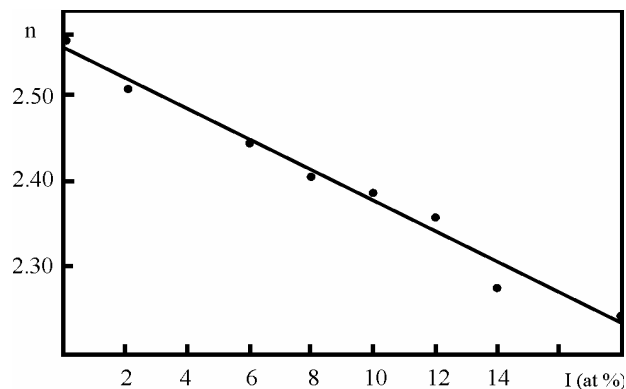
Fig. 17. Dependence of the refractive index on percentage of iodine in the sample.
