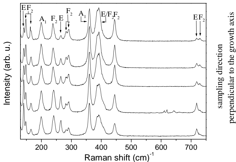
Fig. 1. Raman spectra of \text{Bi}_4\text{Ge}_3\text{O}_{12} , showing a continuous decrease in the F_2 intensity and increase in the E intensity along the sampling line.
