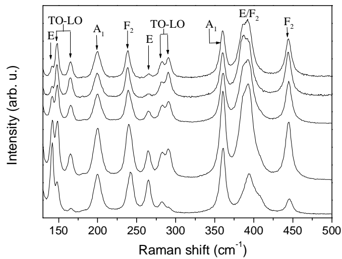
Fig. 2. Raman spectra from selected spots of the \text{Bi}_4\text{Ge}_3\text{O}_{12} crystal, showing variations in the TO/LO intensity ratio of the F_2 modes. The top two spectra were taken from a sampling series along the growth axis, and the lower three spectra from one with a sampling direction perpendicular to the growth axis.
