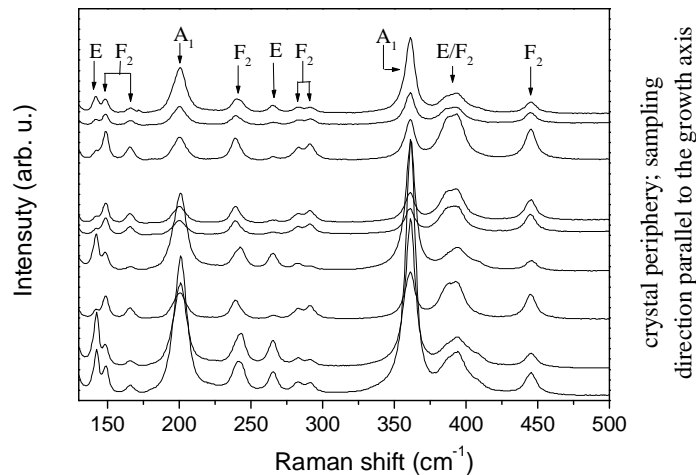
Fig. 3. Raman spectra from the periphery of the \text{Bi}_4\text{Ge}_3\text{O}_{12} crystal, showing sporadic enhancement of the A_1 intensity along the sampling line.
