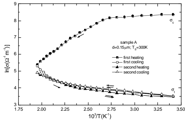
Fig. 2. Typical temperature dependence of the electrical conductivity during heating/cooling cycles for CdO films deposited at 300 K.
