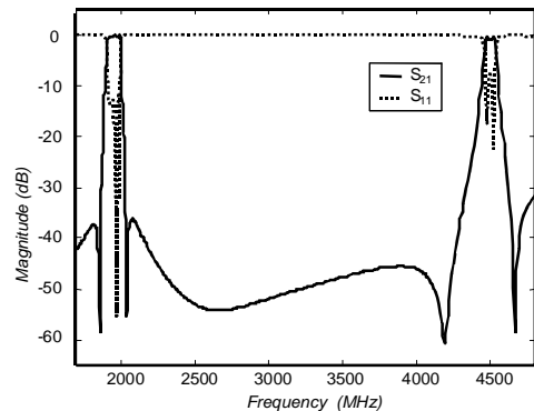
Fig. 5. Simulated wide-band response of the first filter model shown in Fig. 2.
