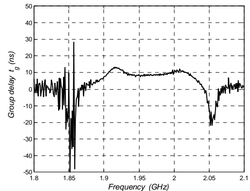
Fig. 4. Measured group delay of the first filter model shown in Fig. 2.
