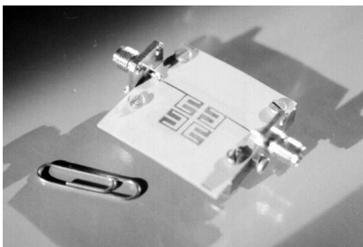
Fig. 2. The first model of the four-pole cross-coupled band-pass filter for UMTS systems.
