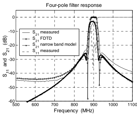
Fig. 12. The frequency response of the four-pole GSM / GPRS filter.
