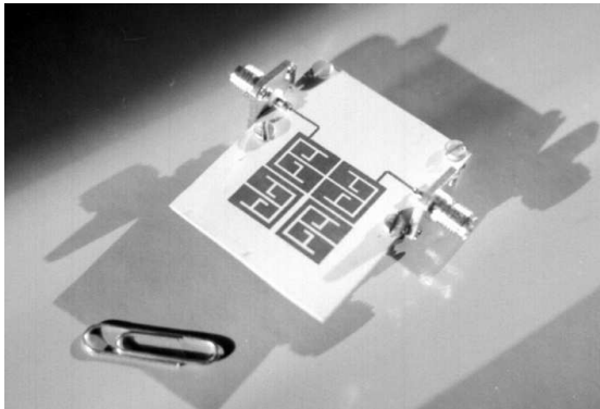
Fig. 11. A four-pole band-pass filter with compact cross-coupled resonators for 900 MHz GSM/GPRS systems.
