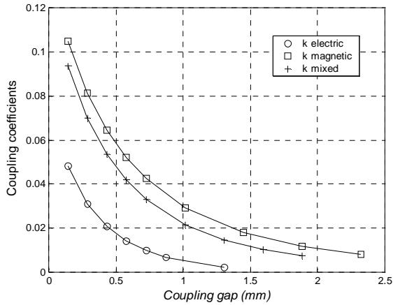
Fig. 1. The coupling coefficients versus the coupling gap for a zero offset.
