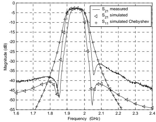
Fig. 3. Measured and simulated frequency response of the first filter model shown in Fig. 2.
