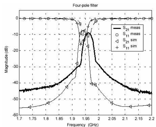
Fig. 10. The measured and simulated frequency responses of the third model of the UMTS cross-coupled filter.
