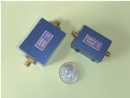
Fig. 15. Encapsulated filters for GSM / GPRS and for UMTS systems, respectively.
