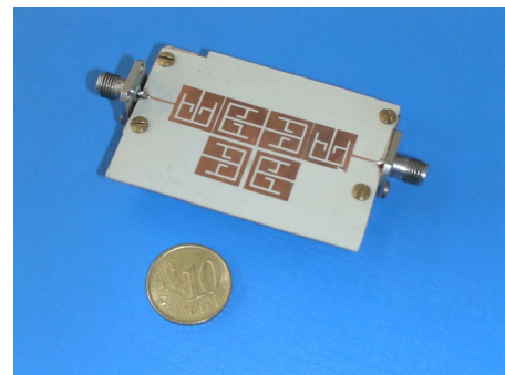
Fig. 13. A six-pole band-pass filter for 900 MHz GSM / GPRS systems.
