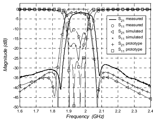
Fig. 7. The comparison between the measured, simulated and prototype responses of the second UMTS filter model.
