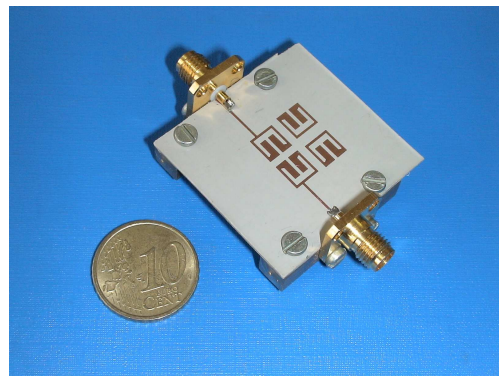
Fig. 9. The third model of the UMTS filter with a narrow pass-band.
