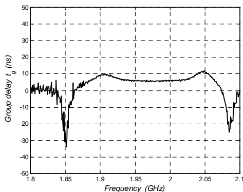
Fig. 8. Measured group delay of the second UMTS band-pass filter model.
