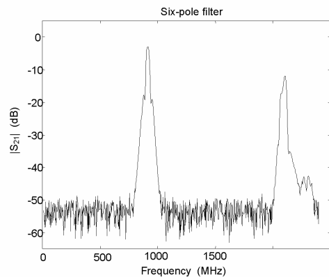
Fig. 14. The measured frequency response of the six-pole GSM / GPRS filter.
