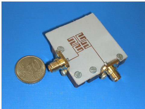
Fig. 6. The second model of the band-pass filter for UMTS systems.
