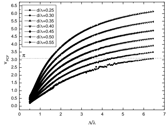
Fig. 3. Numerical results for V parameter with different air-hole diameter (from the bottom, d/\Lambda = 0.3, 0.35, 0.4, 0.45, 0.5, 0.55 ).
