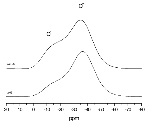
Fig. 4. ^{31}\text{P} MAS NMR spectra of the (100-x)[50\text{P}_2\text{O}_5\cdot 30\text{CaO}\cdot 20\text{Na}_2\text{O}]\cdot x\text{Ag}_2\text{O} glasses.
