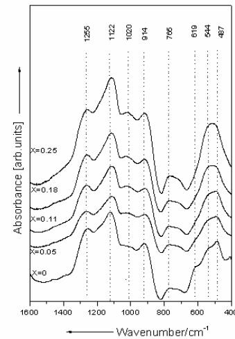
Fig. 3. IR spectra of (100-x)[50\text{P}_2\text{O}_5\cdot 30\text{CaO}\cdot 20\text{Na}_2\text{O}]\cdot x\text{Ag}_2\text{O} glasses.
