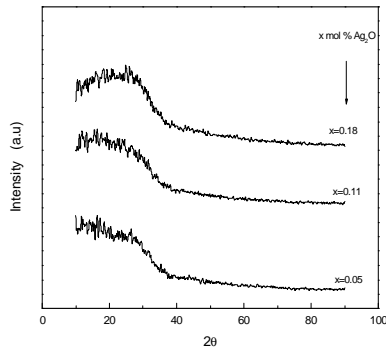
Fig. 1. XDR patterns (100-x)[50\text{P}_2\text{O}_5\cdot 30\text{CaO}\cdot 20\text{Na}_2\text{O}]\cdot x\text{Ag}_2\text{O} samples.
