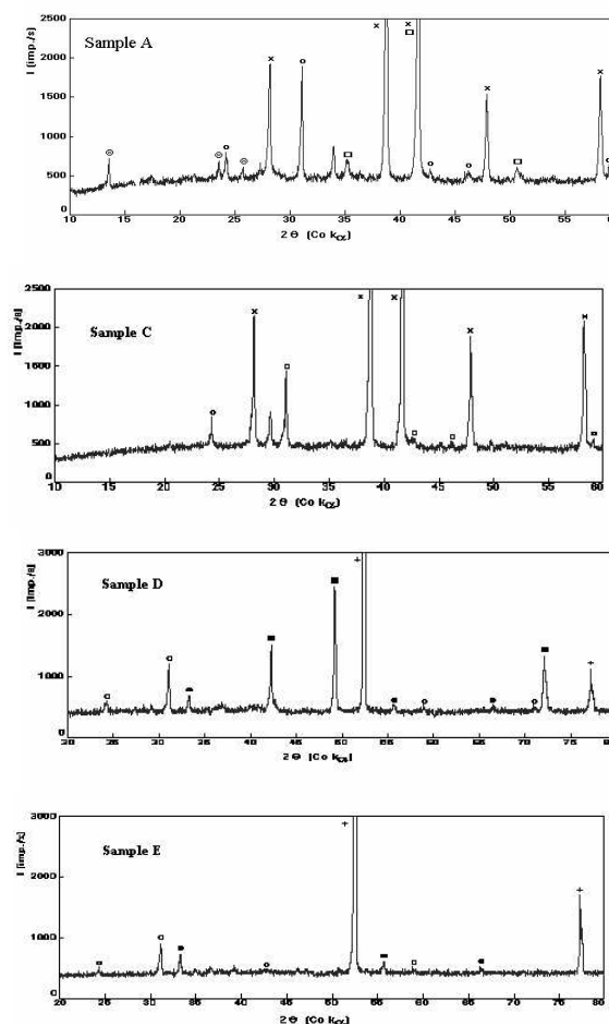
Fig. 1. XRD spectra of samples: A, C, D, E.
