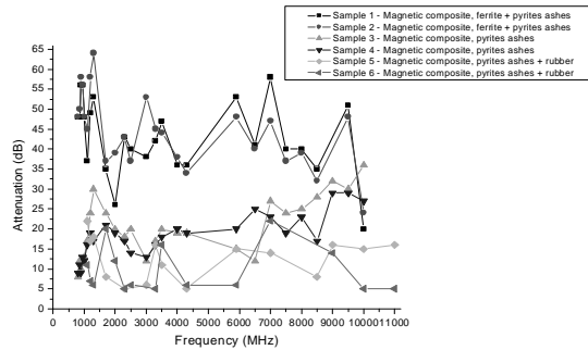
Fig. 2. The attenuation vs. frequencies, for magnetic shields obtained from 50 % ferrite + 50 % pyrites ashes, 100 % pyrites ashes, and pyrites ashes + rubber.
