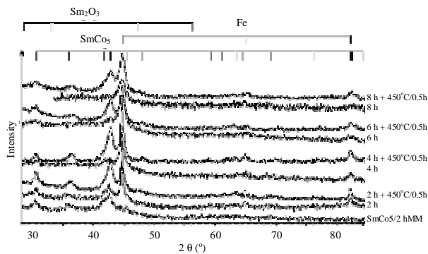
Fig. 1. X-ray diffraction patterns of the \text{SmCo}_5 + 20\% \text{Fe} composite samples for as milled samples (2, 4, 6 and 8 hours of milling) and samples annealed for 0.5 hours at 450^\circ\text{C} , compared to that of \text{SmCo}_5 milled for 2 hours.
