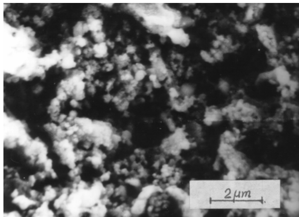
Fig. 3. SEM micrograph for the ferrite MgMn_{0.2}Fe_{1.8}O_4 treated at 1000 °C for 30 minutes.
