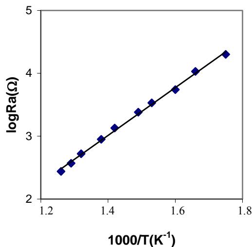
Fig. 4. \log R_a vs. 1/T for studied sample.
