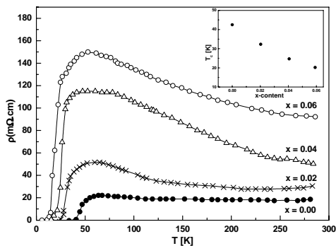
Fig. 2. Temperature dependence of the resistivity for \text{Ru}_{1-x}\text{Sb}_x\text{Sr}_2(\text{Eu}_{0.7}\text{Ce}_{0.3})_2\text{Cu}_2\text{O}_{10-\delta} samples with 0 \leq x \leq 0.06 . Insert T_c vs. content of Sb.
