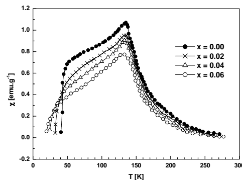
Fig. 4. Temperature dependence of magnetic susceptibility of \text{Ru}_{1-x}\text{Sb}_x\text{Sr}_2(\text{Eu}_{0.7}\text{Ce}_{0.3})_2\text{Cu}_2\text{O}_{10-\delta} samples with 0 \leq x \leq 0.06 .
