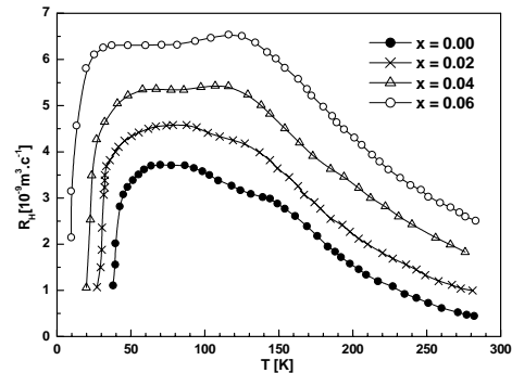
Fig. 3. Temperature dependence of Hall coefficient for \text{Ru}_{1-x}\text{Sb}_x\text{Sr}_2(\text{Eu}_{0.7}\text{Ce}_{0.3})_2\text{Cu}_2\text{O}_{10-\delta} samples with 0 \leq x \leq 0.06 .
