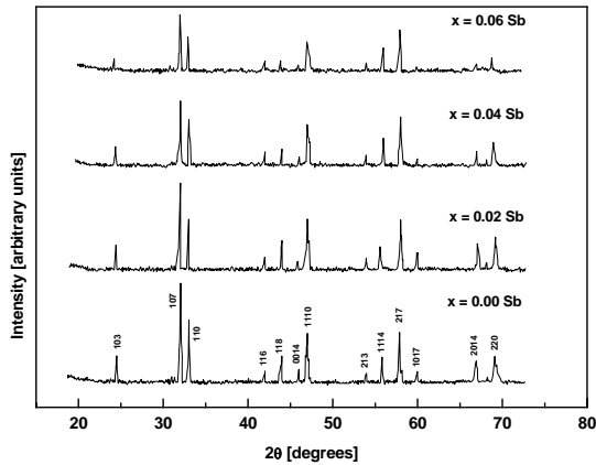
Fig. 1. XRD pattern of \text{Ru}_{1-x}\text{Sb}_x\text{Sr}_2(\text{Eu}_{0.7}\text{Ce}_{0.3})_2\text{Cu}_2\text{O}_{10-\delta} samples with 0 \leq x \leq 0.06 .
