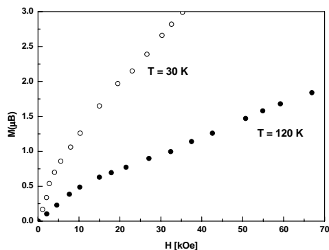
Fig. 5. Field dependence of magnetization for \text{RuSr}_2(\text{Eu}_{0.7}\text{Ce}_{0.3})_2\text{Cu}_2\text{O}_{10-\delta} sample.
