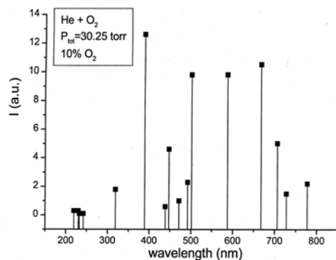
Fig. 6. Emission spectrum of (He+10%O 2 ) gas mixture in a PDP type discharge.
