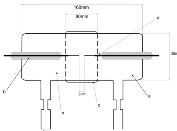
Fig. 4. The experimental set-up for D.C. discharge. a. pyrex discharge tube, b. glass cover, c. wolfram electrodes \Phi 1.5 mm, d. Pyrex capillary tubes \Phi 6.0 mm.
