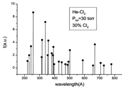
Fig. 11. Emission spectrum of (He+30%Cl 2 ) gas mixture in a PDP type discharge.
