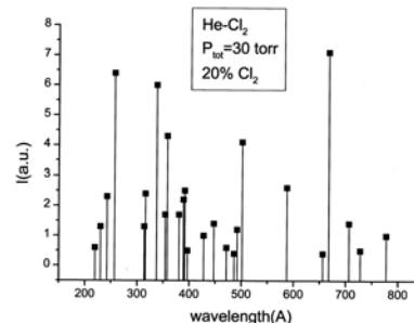
Fig. 10. Emission spectrum of (He+20%Cl 2 ) gas mixture in a PDP type discharge.
