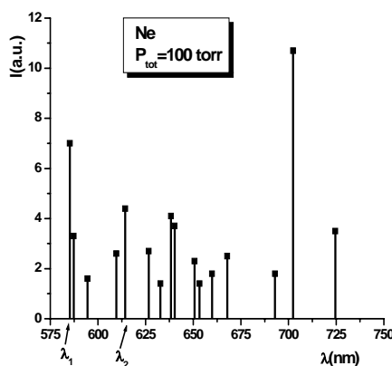
Fig. 1. Recorded spectrum of pure neon PDP discharge ( \lambda_1=585.3 nm, \lambda_2=614.3 nm).
