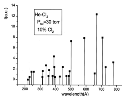
Fig. 9. Emission spectrum of (He+10%Cl 2 ) gas mixture in a PDP type discharge.
