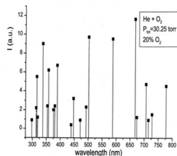
Fig. 7. Emission spectrum of (He+20%O 2 ) gas mixture in a PDP type discharge.
