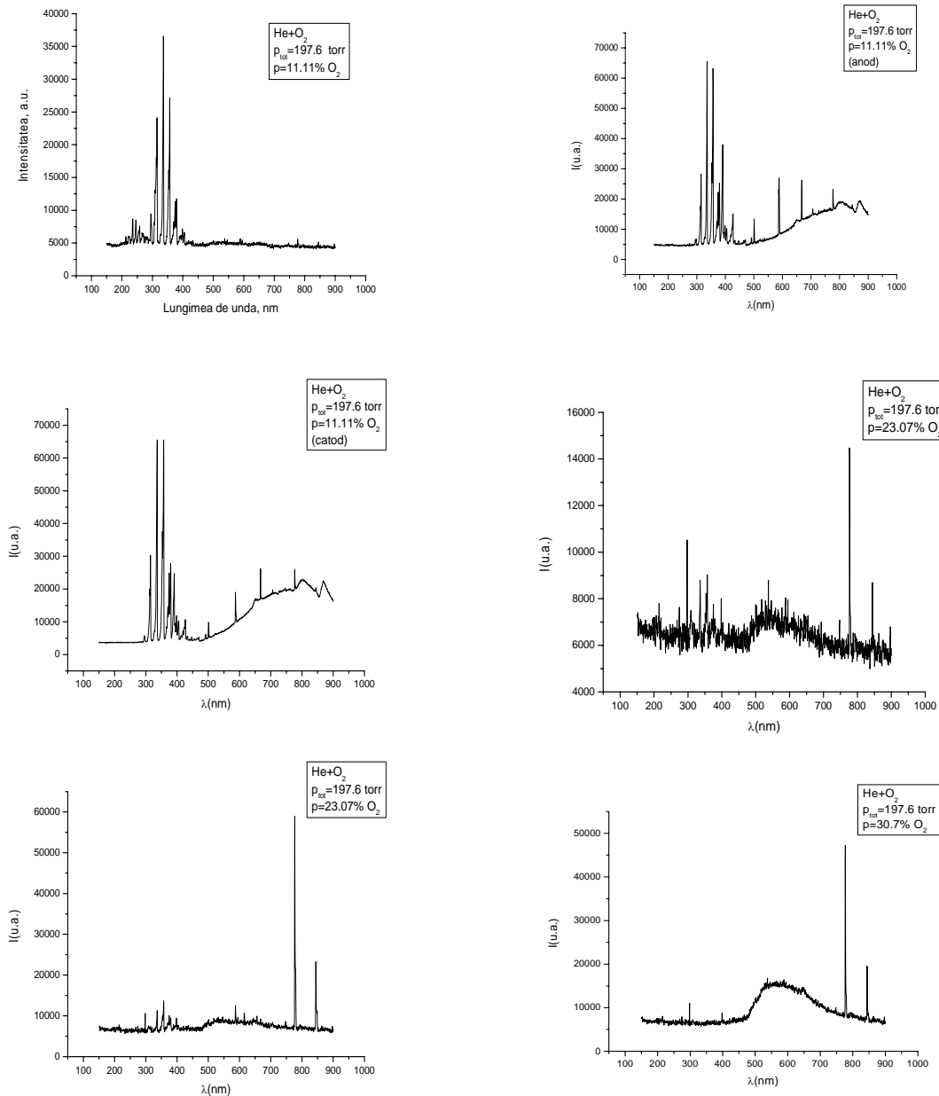
Fig. 12. The emission spectra of a (He+O 2 ) gas mixture D.C. discharge at a total pressure of 197.6 torr for different percentages of electronegative gas.
