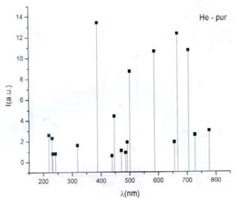
Fig. 5. Emission spectrum of pure helium in a PDP type discharge.
