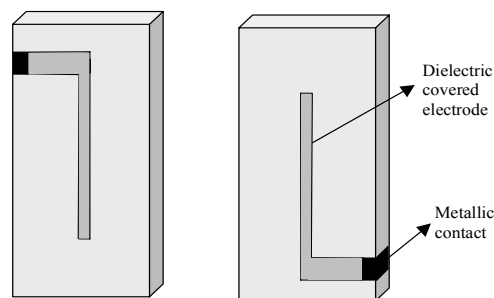
Fig. 3. A view of the deposited thin film electrodes on glass plates.
