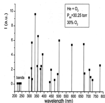
Fig. 8. Emission spectrum of (He+30%O 2 ) gas mixture in a PDP type discharge.
