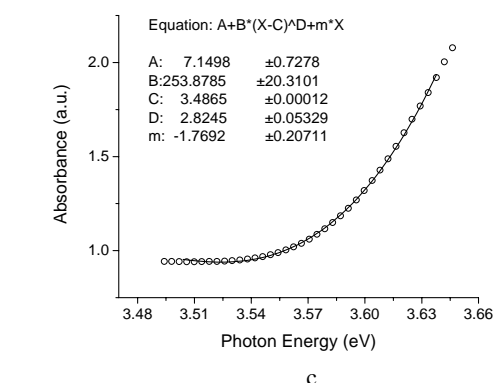
Fig. 6. a) Absorption spectrum of benzil film between: 2.6÷3.3 eV. b), c) Experimental data fitting for film of pure benzil using function (1) for two different energy ranges: b) 2.6÷3.1 eV; c) 3.49÷3.65 eV.
