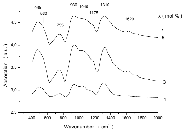
Fig. 3. Infrared spectra of the xMnO(1-x)[3P_2O_5-CaO] glasses.
