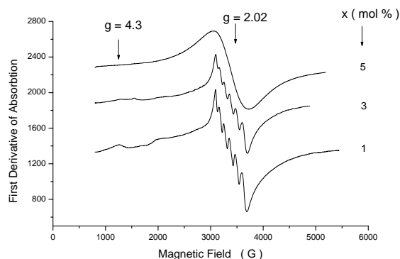
Fig. 1. EPR spectra for x\text{MnO}\cdot(1-x)[3\text{P}_2\text{O}_5\cdot\text{CaO}] glasses.
