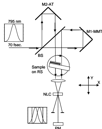
Fig. 2. Sketch of the experimental set-up. The M1-MMT mirrors are mounted on a manual micrometric translation stage with a 10 \mu\text{m} sensitivity. The M2-AT mirrors are mounted on an automatic motorized translation stage with sub-micrometric sensitivity.
