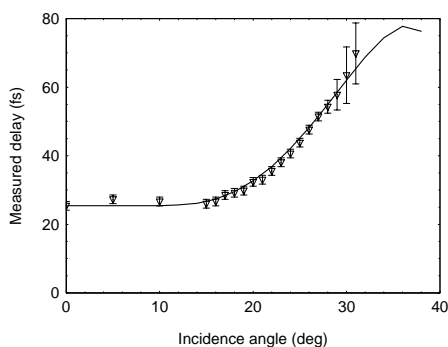
Fig. 3. Measured delay time felt by the incoming pulses as a function of the incidence angle. The experimental data are compared with the numerical calculation of the delay time (solid line).
