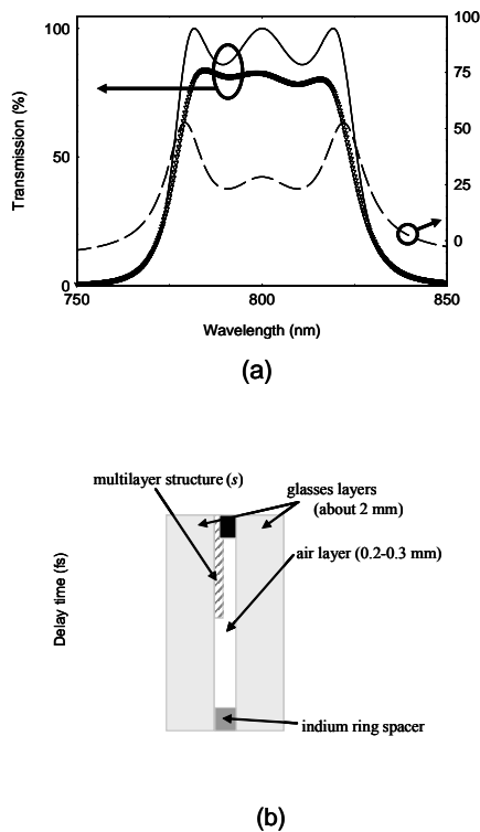
Fig. 1. (a) Theoretical transmission spectrum of the PC structure (thin solid line) at normal incidence together with the experimental spectrum of the fabricated sample (open triangles). With the dashed line is represented the calculated group delay time. [the data are reproduced from the curves in ref.12] (b) Sketch of the test structure. The PC layers are growth only on half of the substrate in order to compare the delay due to the PC with respect to the air gap delay.
