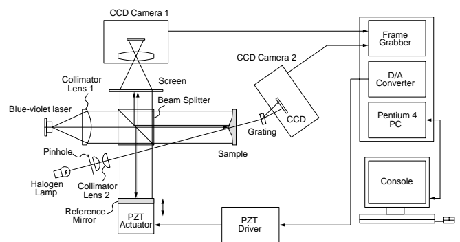
Fig. 1. In-situ simultaneous measuring system of PD and PVC based on the combination of phase-shifting interferometer and computer controlled spectroscopie.
