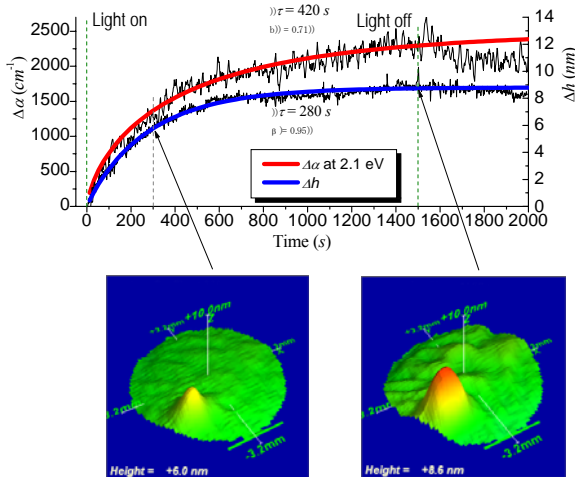
Fig. 5. Time evolution of the \Delta\alpha and \Delta h for \alpha -As 2 Se 3 film ( \lambda = 635 nm, 100 mW/cm 2 ), and height maps at 300 s and 1500 s after illumination starts.
