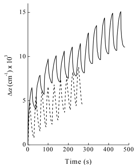
Fig. 3. \Delta\alpha with time for short-duration illumination for a\text{-As}_2\text{Se}_3 films at 50 (solid line) and 300 K (dashed line).
