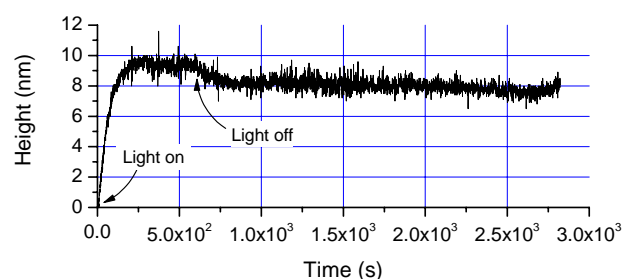
Fig. 4. Time evolution of the surface height for a\text{-As}_2\text{Se}_3 films.
