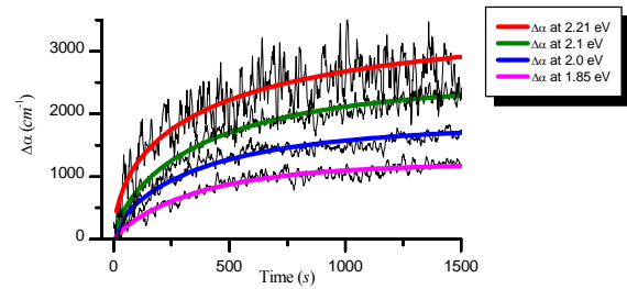
Fig. 6. Time evolution of the \Delta\alpha at various light energies for \alpha -As 2 Se 3 film.
