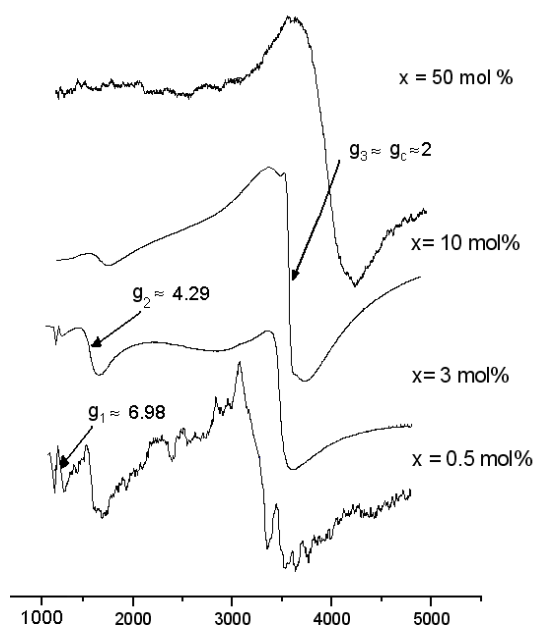
Fig. 1. EPR spectra of \text{Fe}^{3+} ions in x\text{Fe}_2\text{O}_3(100-x)[2\text{P}_2\text{O}_5\text{PbO}] glasses
