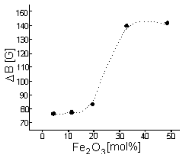
Fig. 2. Linewidth ( \Delta B ) variations vs \text{Fe}_2\text{O}_3 content in x\text{Fe}_2\text{O}_3(100-x)[2\text{P}_2\text{O}_5\text{PbO}] glasses.
