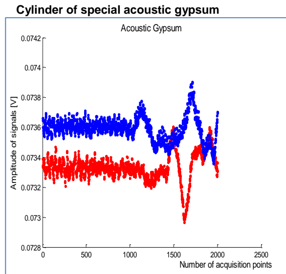
Fig. 9: Diagram for determination of propagation time passing through acoustic gypsum cylinder- Acg
