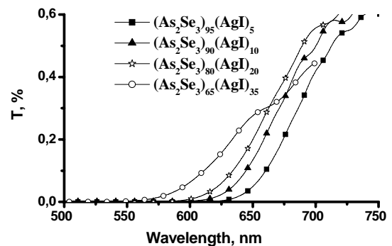
Fig. 3. Transmission spectra of VTE films.
