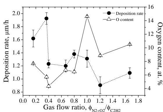
Fig. 1. Deposition rate and oxygen content of the produced Ti-C-O-N coatings as function of the gases flow ratio \Phi(\text{N}_2+\text{O}_2)/\Phi(\text{C}_2\text{H}_2) .
