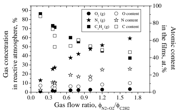
Fig. 3. Reactive gases concentration in deposition chamber (solid symbols) and composition of the produced TiCON coatings (open symbols) as function of the gas flow ratio \Phi(\text{N}_2+\text{O}_2)/\Phi(\text{C}_2\text{H}_2) .
