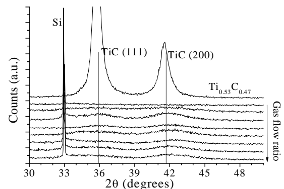
Fig. 4. XRD patterns of Ti-C-O-N coatings as function of gases flow ratio. The XRD pattern in the top corresponds to a coating deposited without nitrogen or oxygen in the chamber and is presented for comparison.
