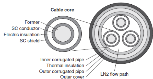
Fig. 10. Structure of the HT c SC cable
