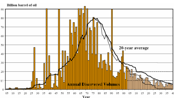
Fig. 2: Confronting the supply challenges, annual discovered volume of oil (1905-2040).
