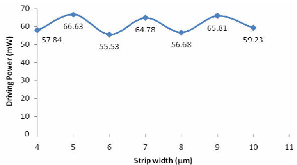
Fig. 9. Driving power versus the width of a straight heater.
