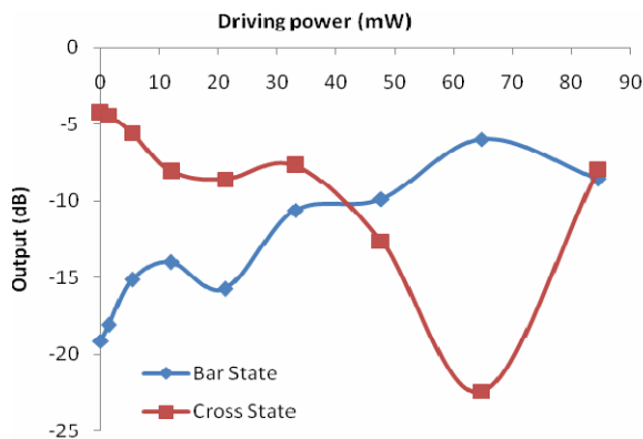
Fig. 7. Switching characteristics of the MMI switch with the straight heating electrode.
