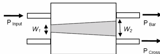
Fig. 6. Schematic configuration of the thermo-optic MMI switch with a thin tapered heating electrode.
