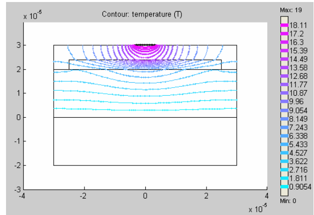
Fig. 5. Temperature distribution in which the straight heater is powered by 0.065 W.
