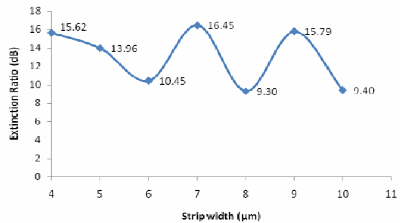
Fig.8. Extinction ratio versus the width of a straight heater.
