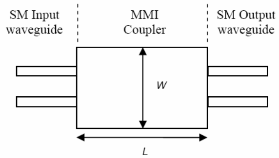
Fig. 2. Layout of the MMI cross coupler
