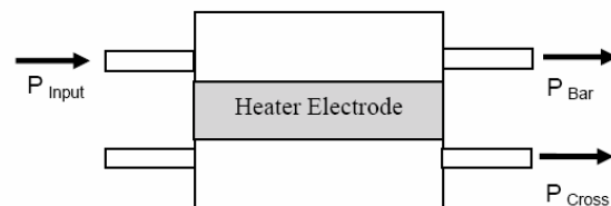
Fig. 3. Schematic configuration of the thermo-optic MMI switch with a straight heating electrode.
