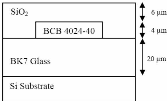
Fig. 1. Cross section of the MMI based cross coupler.
