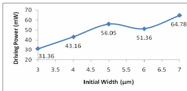
Fig. 10. Driving power versus the initial width of a tapered heater.
