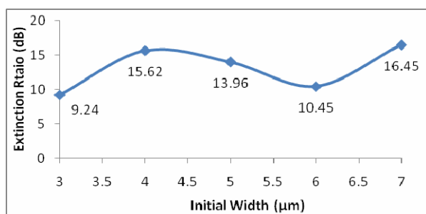
Fig. 11. Extinction ratio versus the initial width of a tapered heater.
