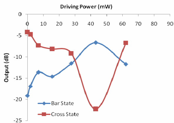
Fig. 12. Switching characteristics of the MMI switch with the tapered heating electrode.
